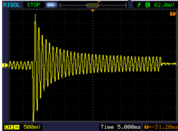
Fig. 7: Slow attack
