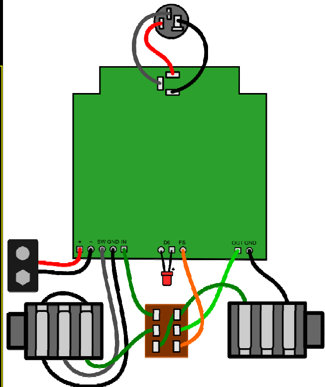
Fig. 3: Wiring diagram (with millennium bypass)
