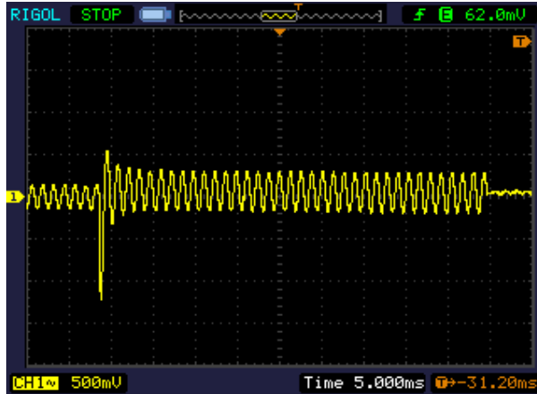
Fig. 6: Fast attack
