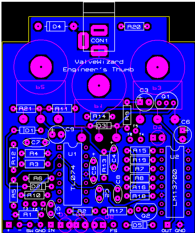
Fig. 2: Component layout
