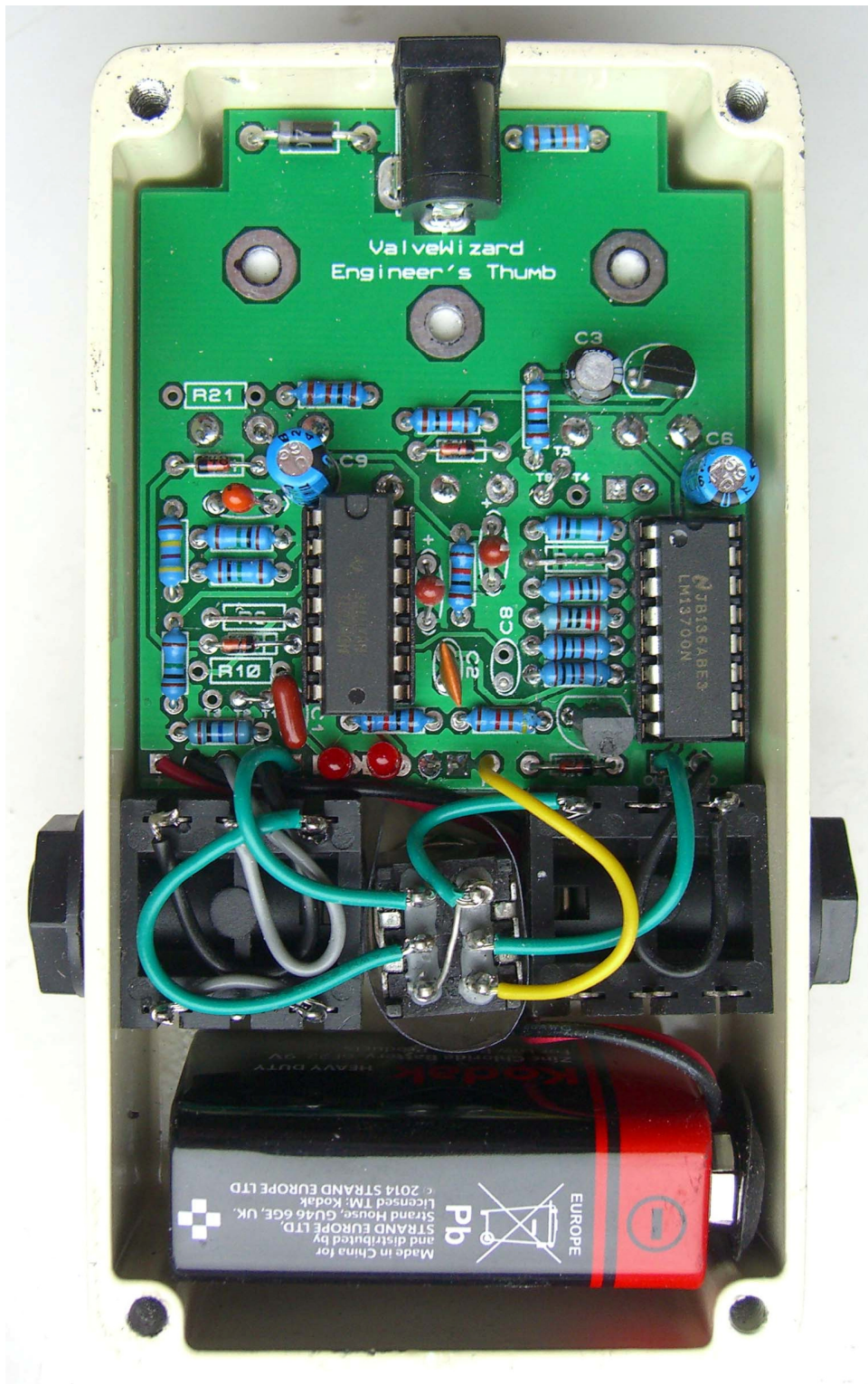
Fig. 5: Close-up of the populated PCB
